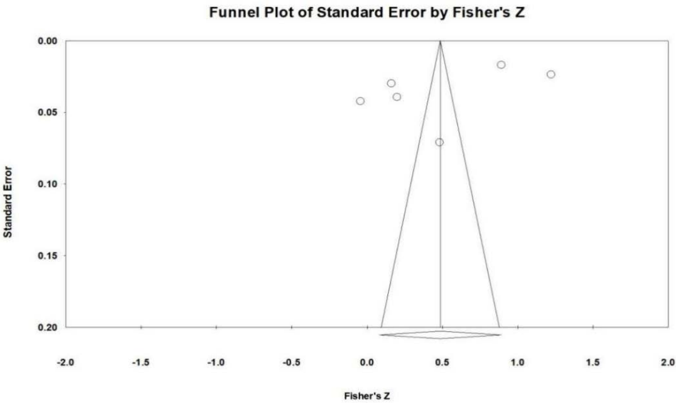
Figure 4 Funnel Scatter Plot for Perceived Teacher Support (PTS)
