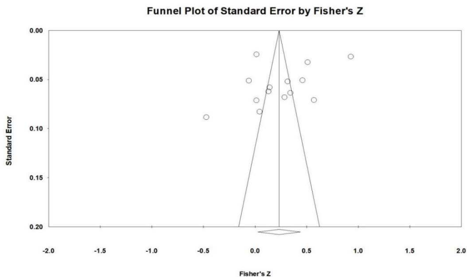
Figure 2 Funnel Scatter Plot for Perceived Social Support (PSS)
