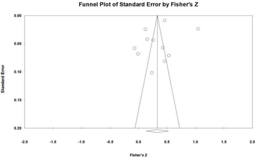
Figure 5 Funnel Scatter Plot for Perceived Peer Support (PPrS)
