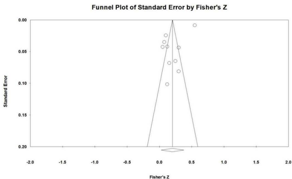
Figure 3 Funnel Scatter Plot for Perceived Parental Support (PPS)
